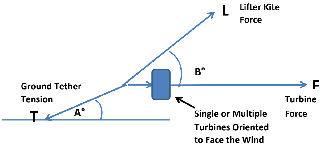
LIFTER TETHER ANGLE ( B^\circ ) = 45^\circ
